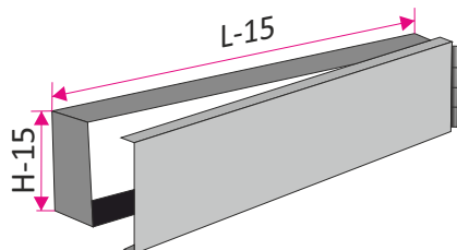
GU - cantilevered damper (especially recommended for grills to spiro channel)
