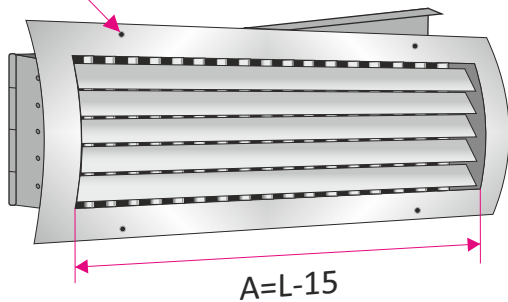
L,H - dimensions of the grille mounting hole
