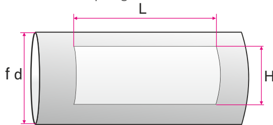
L,H - dimensions of the grille mounting hole
